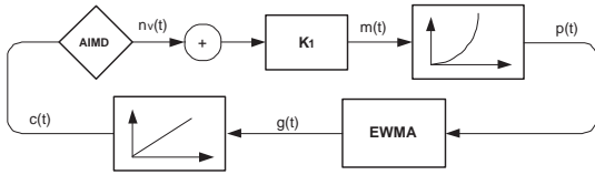
Figure 2: Block diagram for application adaptation
