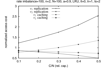
Fig. 9. Analytic results on the comparison of replication and caching under three cases of request imbalance (1,10 and 100).
