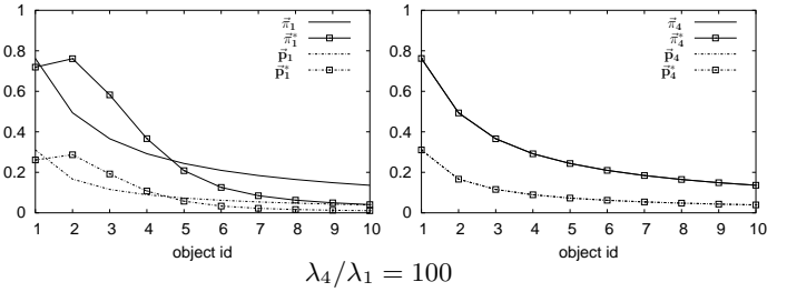
Fig. 5. Analytic results on the repetition of the \lambda_4/\lambda_1 = 100 (third row of Fig. 4) - but this time with a smaller storage capacity C = 3 .
