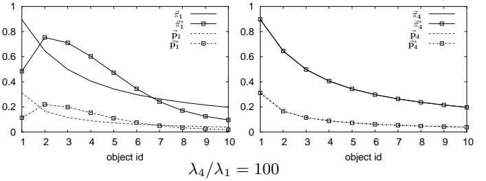
Fig. 4. Analytic results on the effect of request rate imbalance on the per object request and hit probabilities under LRU (values with "*" superscript) and LRU without state interaction. \vec{p} denotes the demand and \vec{\pi} the steady-state hit probabilities. Other parameters: N = 10 , n = 4 , C = 4 , \alpha = 0.9 .
