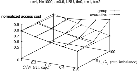
Fig. 6. Analytic results on the effect of the state interaction on the normalized access cost of the overactive node and the remaining nodes of the group under different relative storage capacities and request rate imbalances. No mistreatment occurs in this case.
