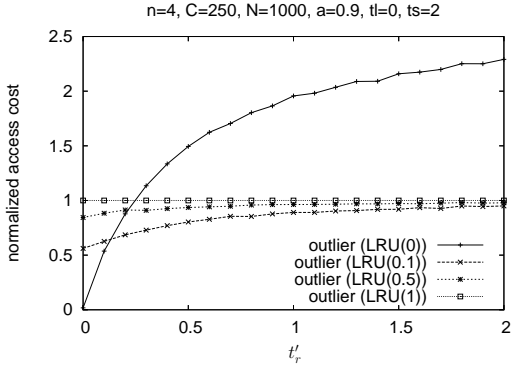
Fig. 16. Simulation results on the effect of the remote access cost t'_r on the normalized access cost of the outlier node under different LRU( q ) schemes.
