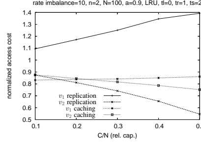
Fig. 9. Analytic results on the comparison of replication and caching under three cases of request imbalance (1,10 and 100).
