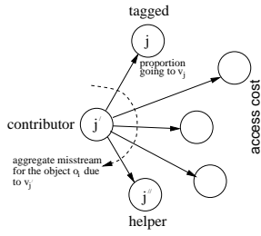
Fig. 2. Graphical illustration for the explanation of Eq. (7).
