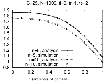
Fig. 3. Validation of the approximate analytic model of Section III-B through comparison with simulation results on the social cost of the group.
