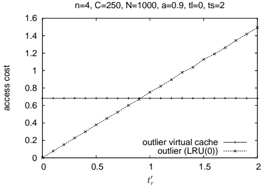
Fig. 17. Simulation results on the effect of the remote access cost t'_r on the access cost of the outlier node under the virtual cache and LRU(0) schemes.
