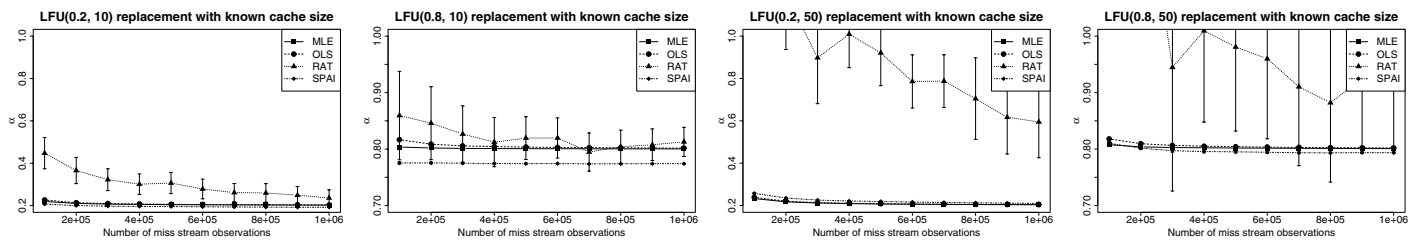
Fig. 1. SPAI vs MLE, OLS, and RAT on inferring the exponent of a GPL from samples of its tail (objects with rank C + 1 and higher) shown with 95% confidence intervals.
