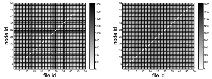
Fig. 4. Maximum finish time for all nodes and all files under Random with cooperative nodes and Max-Min with upload-selfish slowest node ( \frac{k}{n} = 0.04 ).
