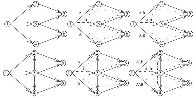
Fig. 1. Mixing max-flows. Left: empty network. Middle: RF(1,5) and RF(1,6) co-existing. Right: RF(1,2) , RF(1,3) , RF(1,4) , RF(1,5) , RF(1,6) co-existing. Top: initial network. Bottom: Initial augmented with edges, (3,2) and (3,4).
