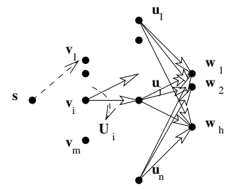
Fig. 6. Reduction from MAX-UNIQUES( k ) to Max-Sum.
