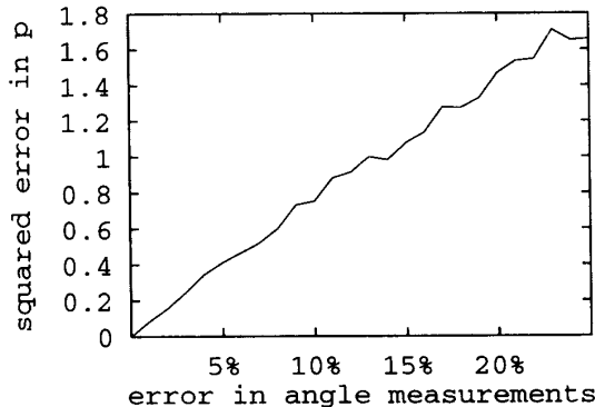
Figure 2: Simulation results using algorithm POSITION ESTIMATOR on an input of noisy angle measurements. The squared error in the position estimate p (in meters) is shown as a function of measurement errors (in percent of actual angle).
