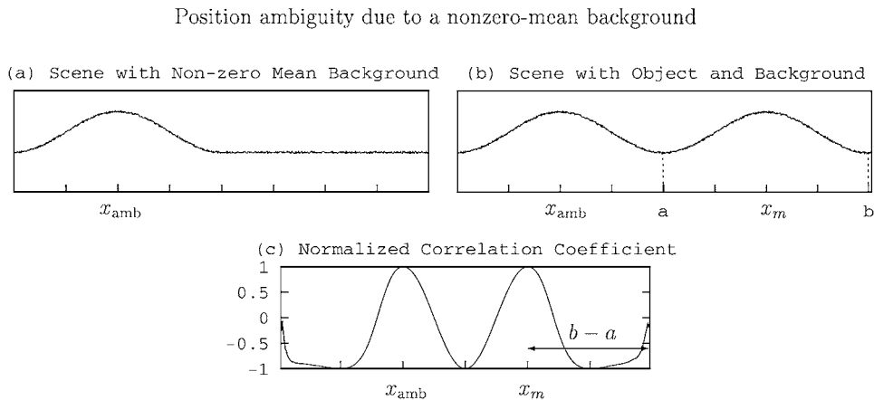
Figure 4. (a) A nonzero-mean scene that, on the left, has background ambiguity with shape identical to the object in Fig. 1(a). (b) The same scene, but on the right, the object occludes the nonzero-mean background between a and b . (c) The normalized correlation coefficient between scene (b) and the object in Fig. 1(a). The position of the object in (b) cannot be estimated unambiguously, since the object could be found either on the left at x_{amb} or on the right at x_m . In typical computer vision scenarios, however, such ambiguity is unlikely, unless the complexity of the scene object is low.
