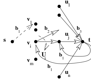
Fig. 5. Reduction from MAX-UNIQUES( k ) to Max-Min.
