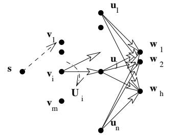
Fig. 6. Reduction from MAX-UNIQUES( k ) to Max-Sum.
