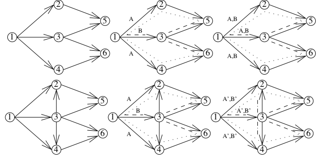
Fig. 1. Mixing max-flws. Left: empty network. Middle: \text{RF}(1,5) and \text{RF}(1,6) co-existing. Right: \text{RF}(1,2) , \text{RF}(1,3) , \text{RF}(1,4) , \text{RF}(1,5) , \text{RF}(1,6) co-existing. Top: initial network. Bottom: Initial augmented with edges, (3,2) and (3,4).
