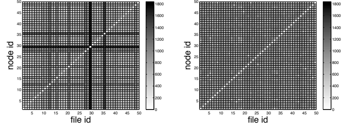
Fig. 4. Maximum finish time for all nodes and all files under Random with cooperative nodes and Max-Min with upload-selfish slowest node ( \frac{A}{n} = 0.04 ).
