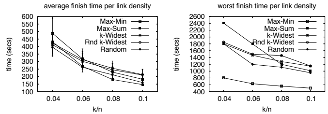
Fig. 3. Simulation of a closed network based on Sprint's topology.
