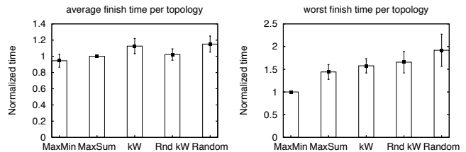
Fig. 2. PlanetLab experiment, mid June 2007.
