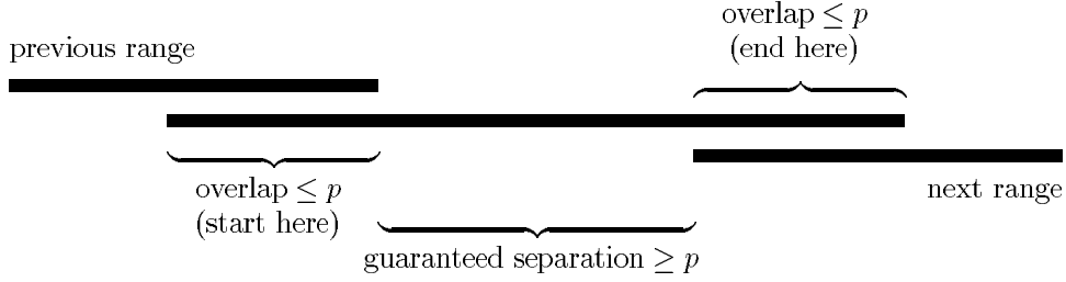
Figure 2. Range of a rightward head
