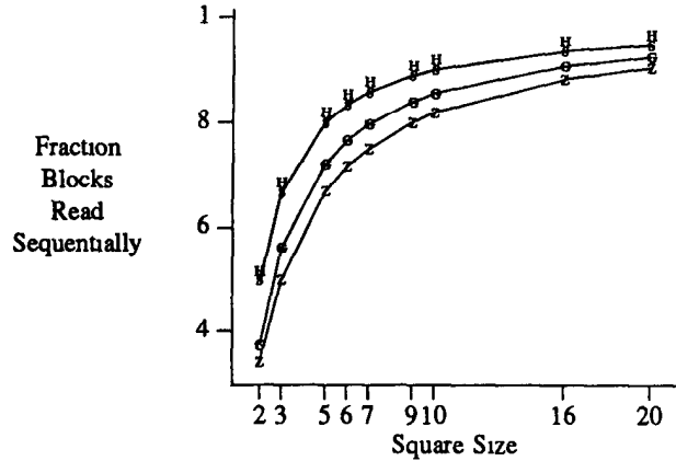
Figure 8. Fraction of blocks (of size 1) read sequentially as the size of the selected square is varied
