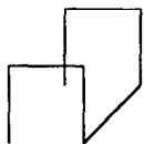
Figure 14. The Primitive for a 3-dimensional Hilbert Curve
