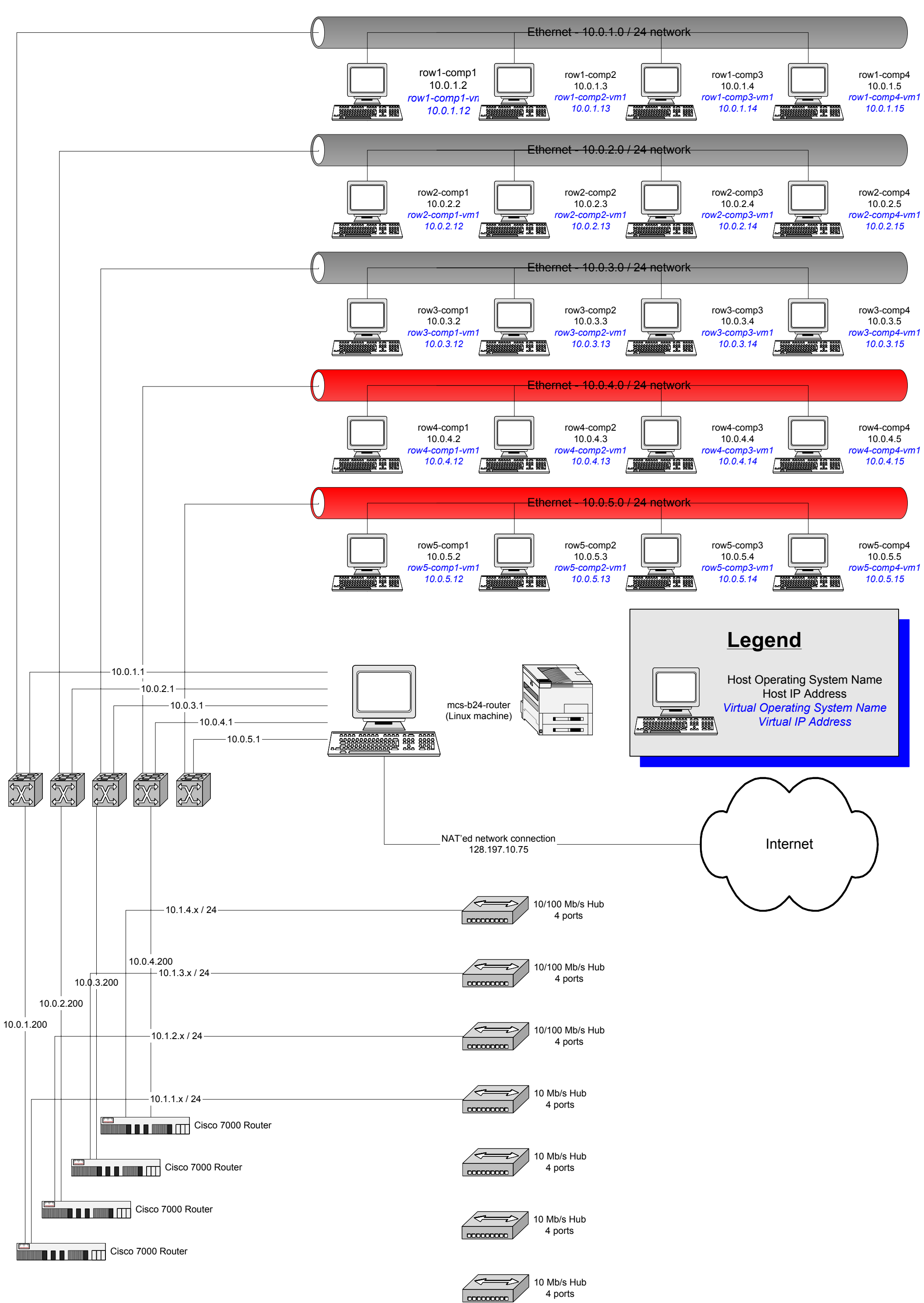
MCS B24 Networking layout
