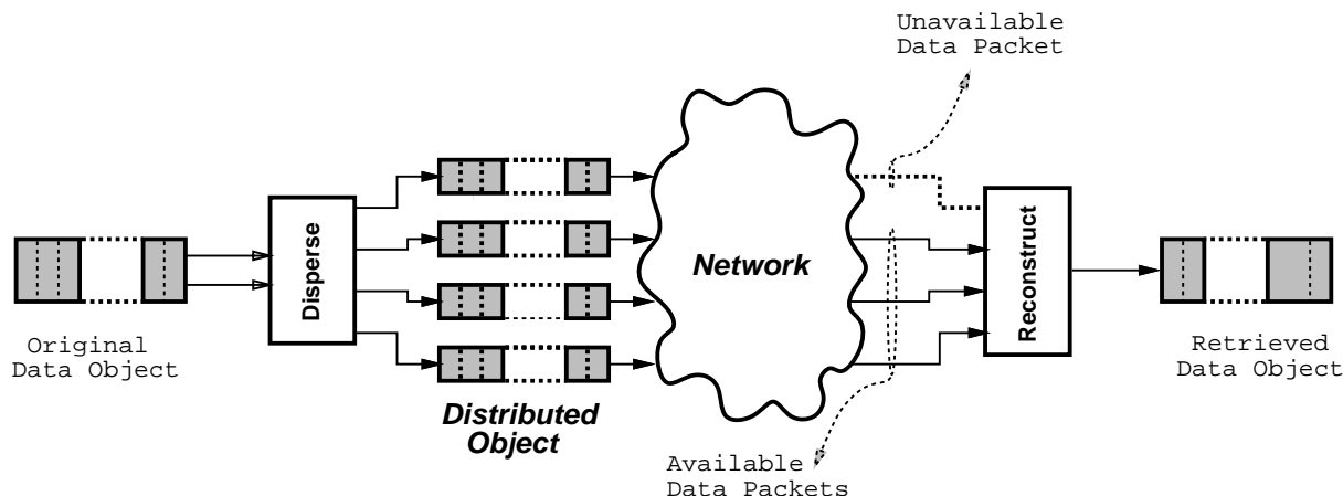
Figure 2: Dispersal and reconstruction of information using IDA.
