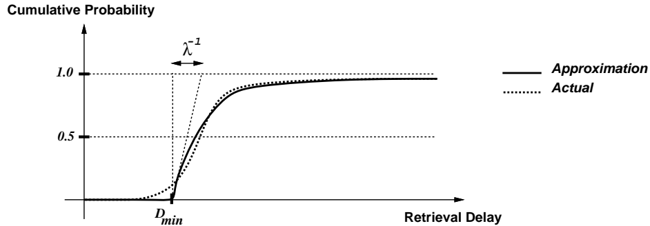
Figure 4: End-to-end delay characteristic function under the exponential delay assumption.
