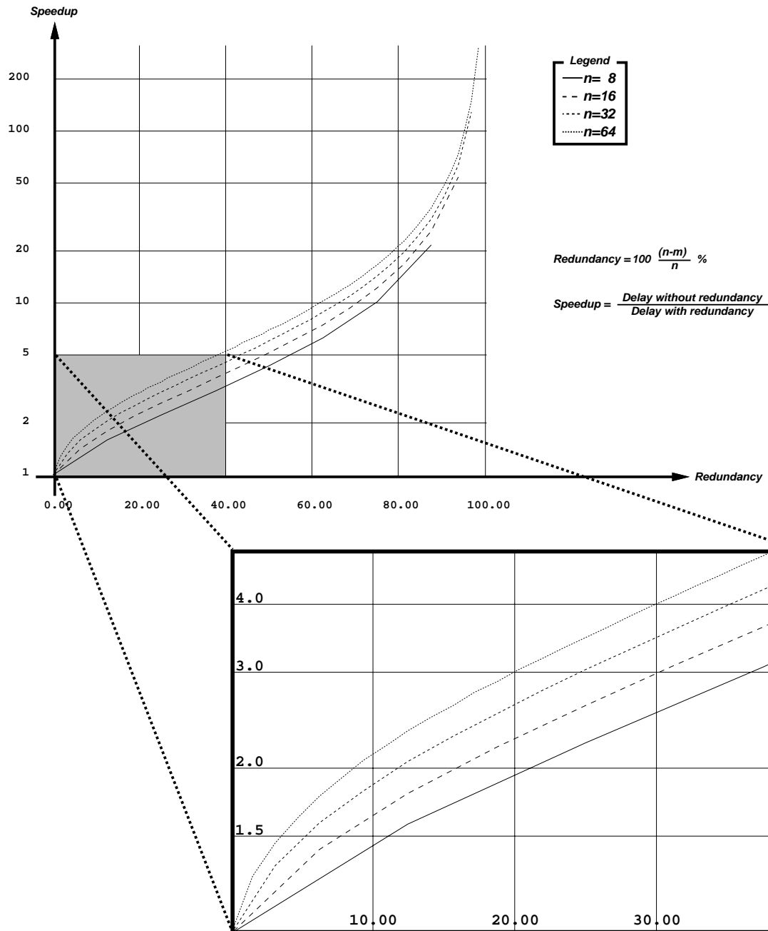
Figure 5: Expected AIDA speedups – Only the random part of the delay is considered.
