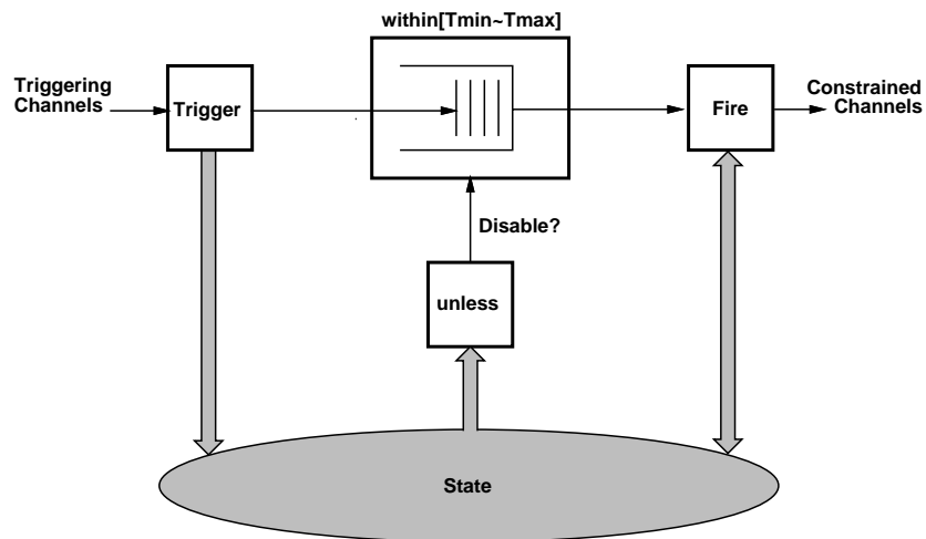
Figure 5: Time-constrained Event-driven Transaction (TET).
