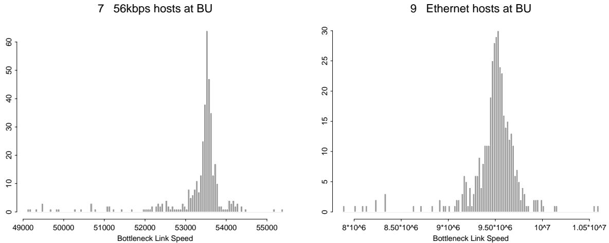
Figure 3: Histograms of BPROBE results. Left: 56Kbps; Right: 10Mbps
