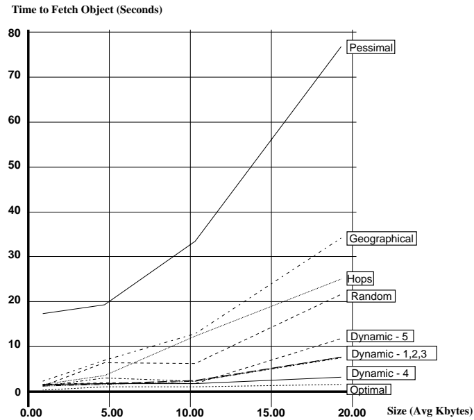
Figure 7: Fetch Times of Static and Dynamic Policies Plotted Against Document Sizes.
