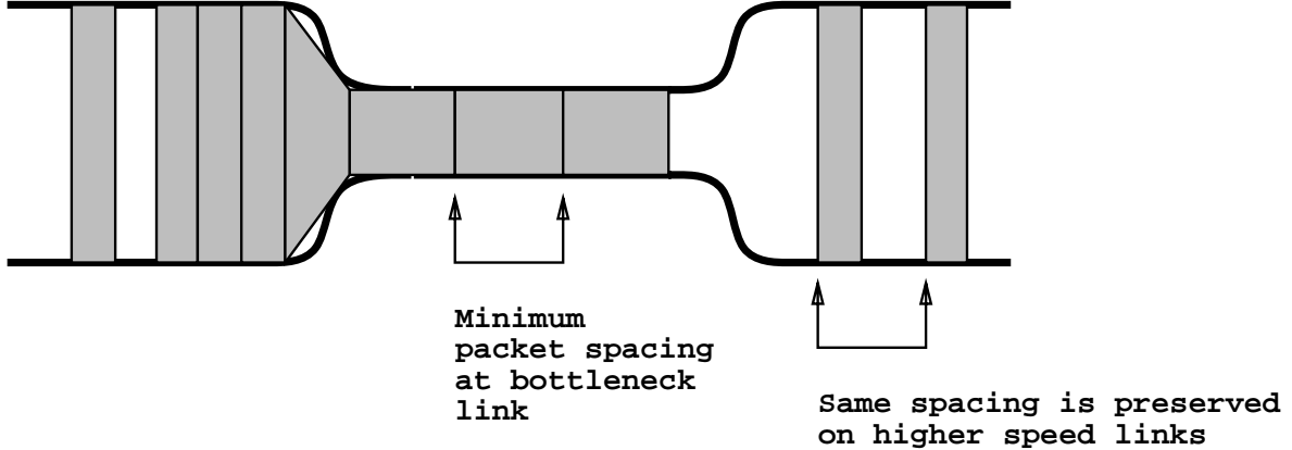
Figure 1: Packet flow through a bottleneck link
