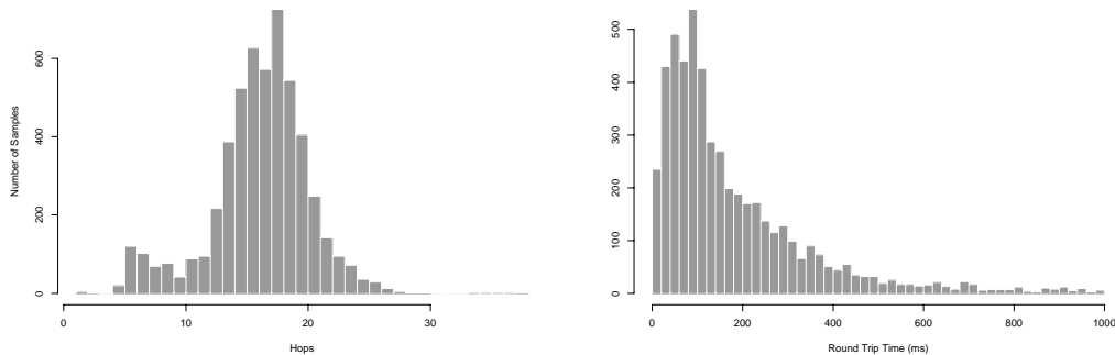
Figure 4: Empirical Distribution of Hops and RTT to 5262 Random Servers
