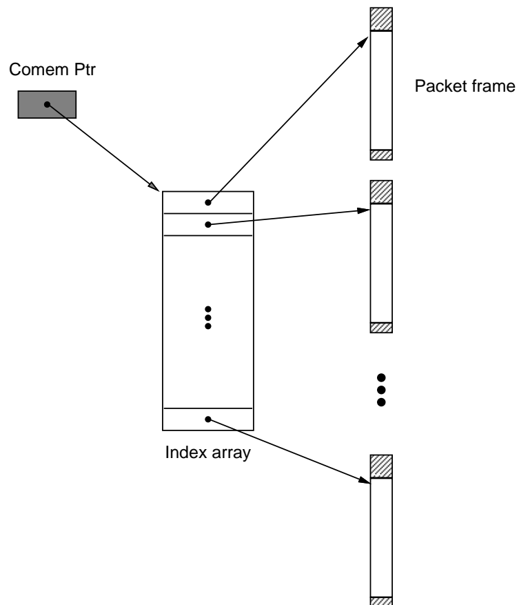
Figure 3: A possible memory layout of a comem region.
