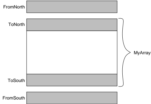
Figure 6: Slice of the array for the DSM example allocated to a single process, shaded areas represent comem regions.
