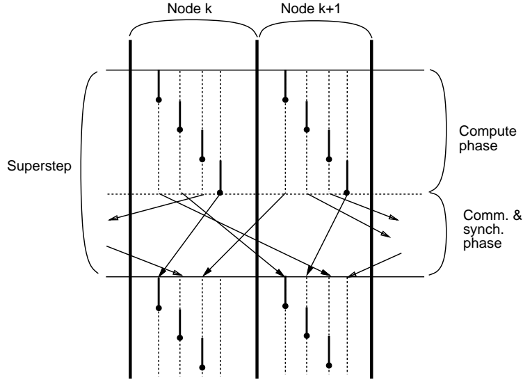
Figure 1: Structure of a BSP computation in which each processor executes four BSP processes. A solid circle represents a barrier invocation, and a solid horizontal line represents its return.
