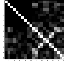
Figure 5: Example of matrix \mathbf{M}^T \mathbf{M} .
