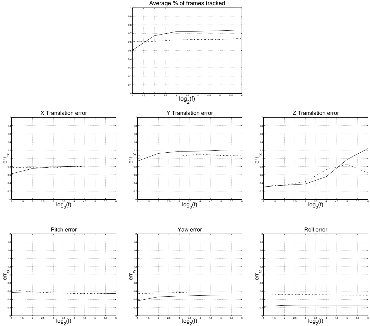
Figure 15: Experiment 4: sensitivity of cylindrical and planar tracker to the focal length. In all the graphs, the solid curve corresponds to the cylindrical tracker and the dashed curve to the planar tracker. The first (top) graph shows the average number of frames tracked over the set of 45 sequences, while varying focal length. The next three graphs show the average error in estimating the x , y and z position, respectively. The bottom three graphs show the average error in estimating the rotation about the x , y and z axes, respectively.
