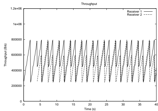
Fig. 6. Asynchronous receivers sharing bottleneck bandwidth
