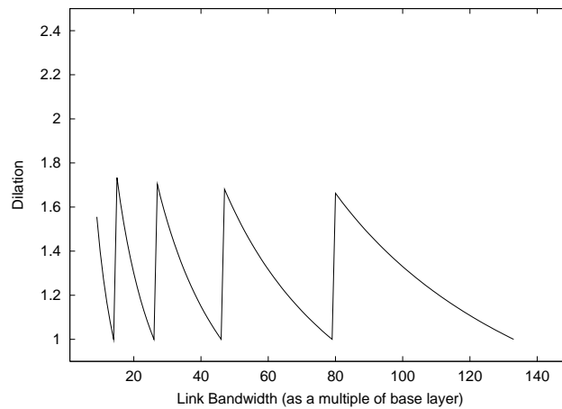
Fig. 2. Maximal dilation at a link as a function of available link bandwidth
