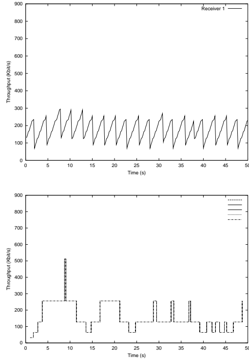
Fig. 4. A comparison of Fib1 (top) and RLC (bottom) multicast congestion control sharing bottleneck bandwidth
