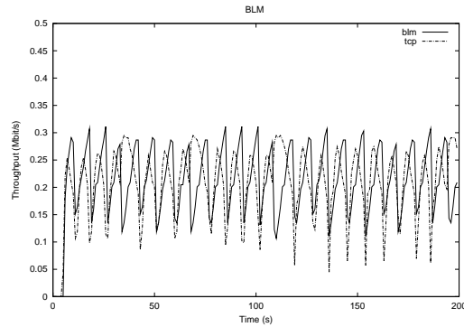
Fig. 5. Fib1 multicast congestion control competing with a TCP flow
