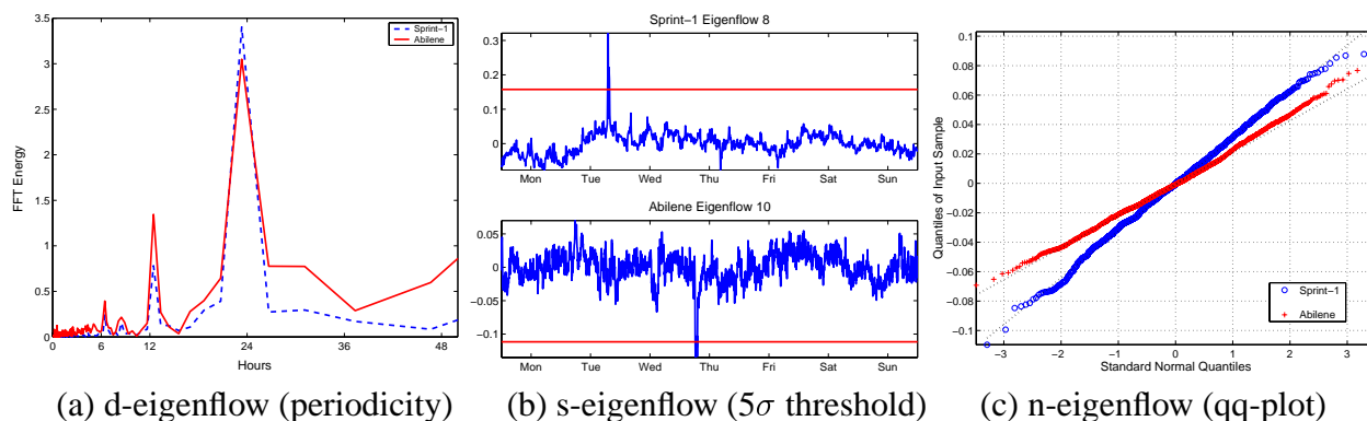
Figure 9: Classifying eigenflows by using three tests.
