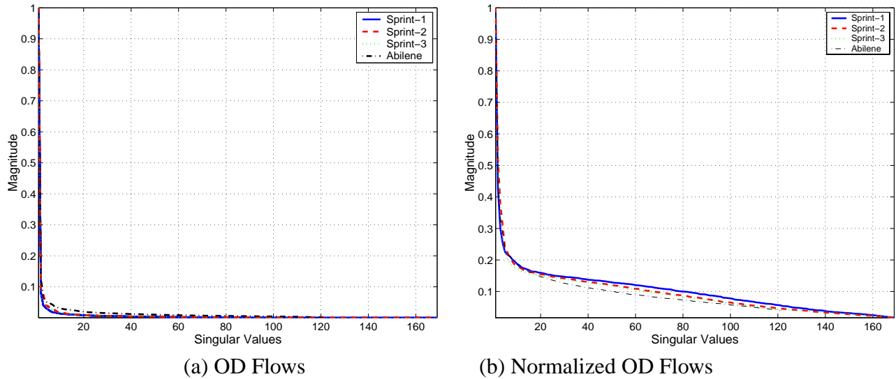
Figure 4: Scree plot for OD flows.
