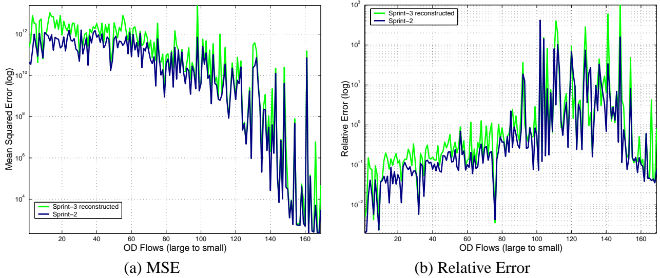
Figure 13: Exploring the temporal stability of Principal Components.
