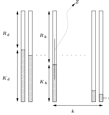
Figure 2: The sets K_k and R_k . A Z gate that involves bits in both sets is shown.
