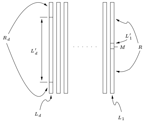
Figure 1: Decomposition of the layers of the circuit C .
