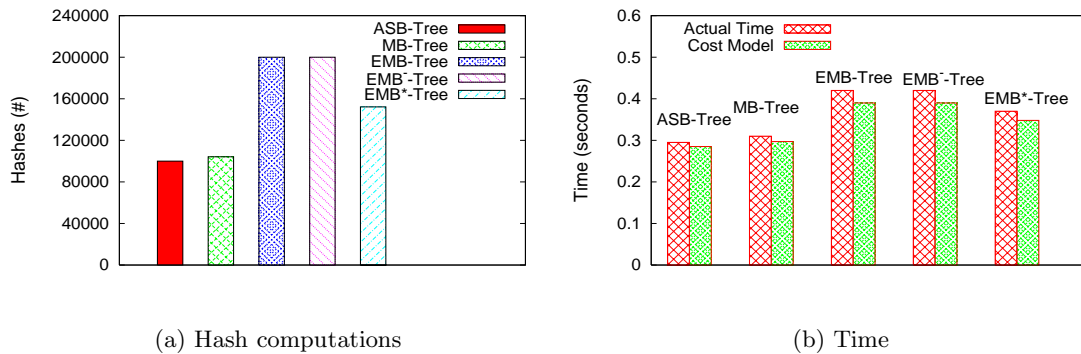
Figure 9: Hash computation overhead.
