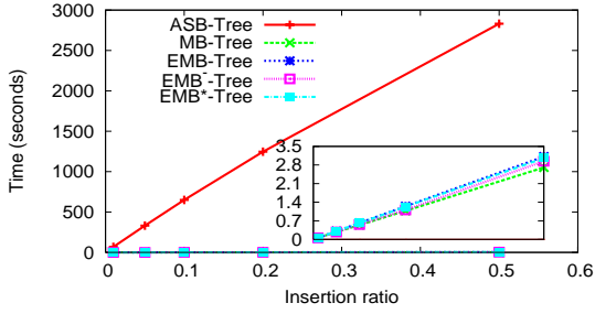
(c) Computation cost.
