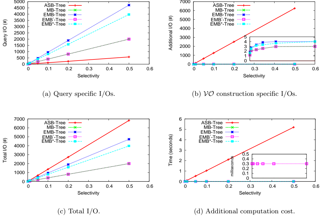
Figure 10: Performance analysis for range queries.
