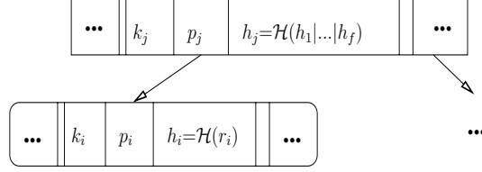
Figure 3: An MB-tree node.
