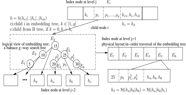
Figure 6: An EMB^* -tree node.
