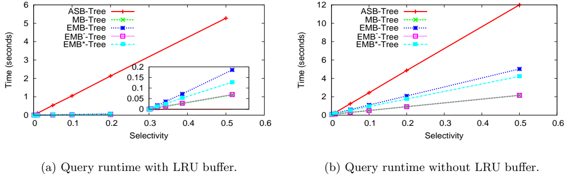
Figure 11: The effect of the LRU buffer.
