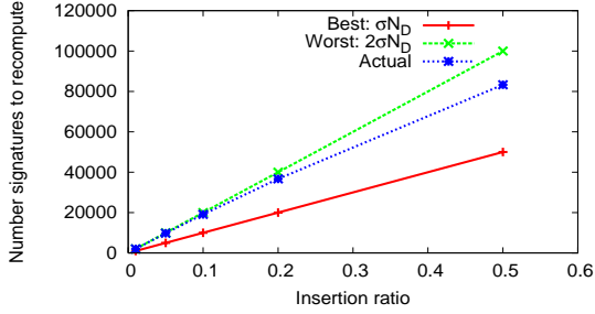
(a) Number of signature re-computations.
