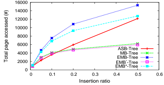
(b) Number of pages affected.
