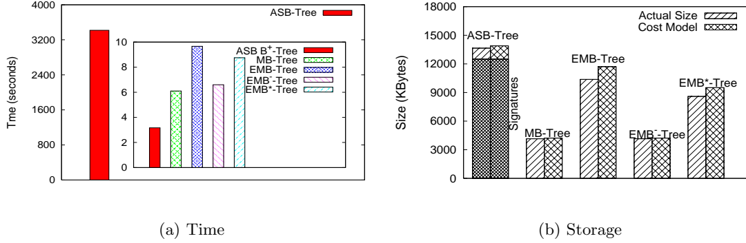
Figure 8: Index construction cost.
