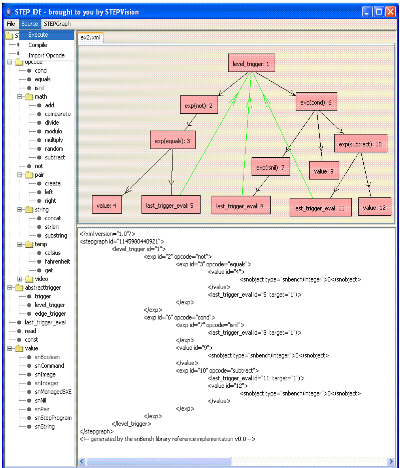
Figure 3: A screen-shot of "STEPVIEW".
