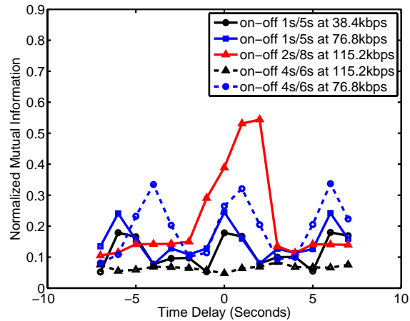
Figure 6-3: Rate Scheduler's Sensitivity to Buffer Occupancy
