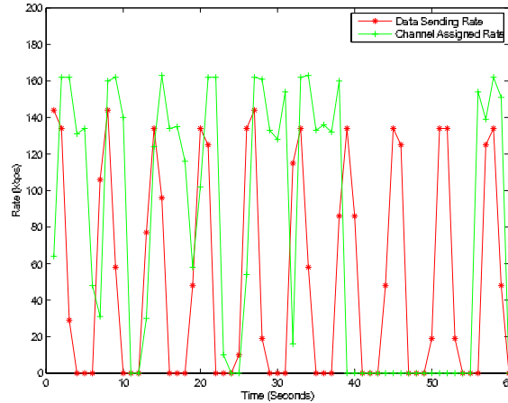
Figure 6-9: Channel Scheduler Tracking an On-Off Data Source with Peak Rate of 153.6 kbps
