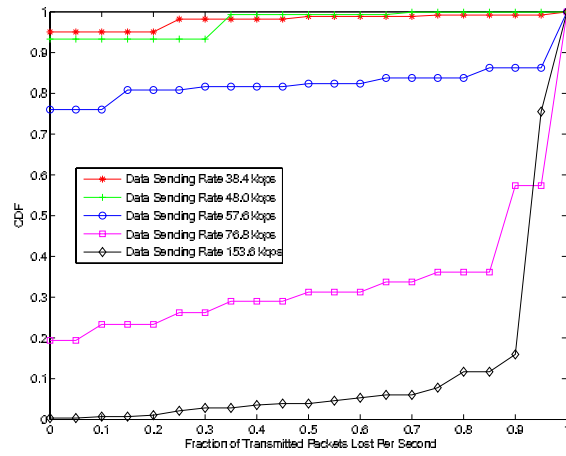
Figure 6-12: CDF of the Fraction of Packets Lost Per Second for UDP CBR Experiments
