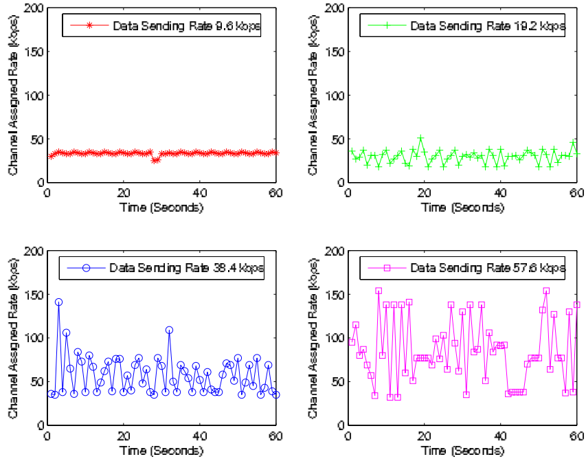
Figure 6-8: Time Series of Assigned Channel Rate for UDP CBR Experiments
