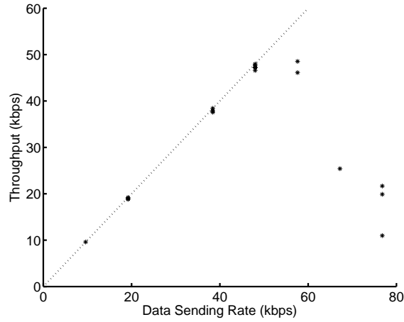
Figure 6-1: Average Throughput for UDP CBR Experiments
