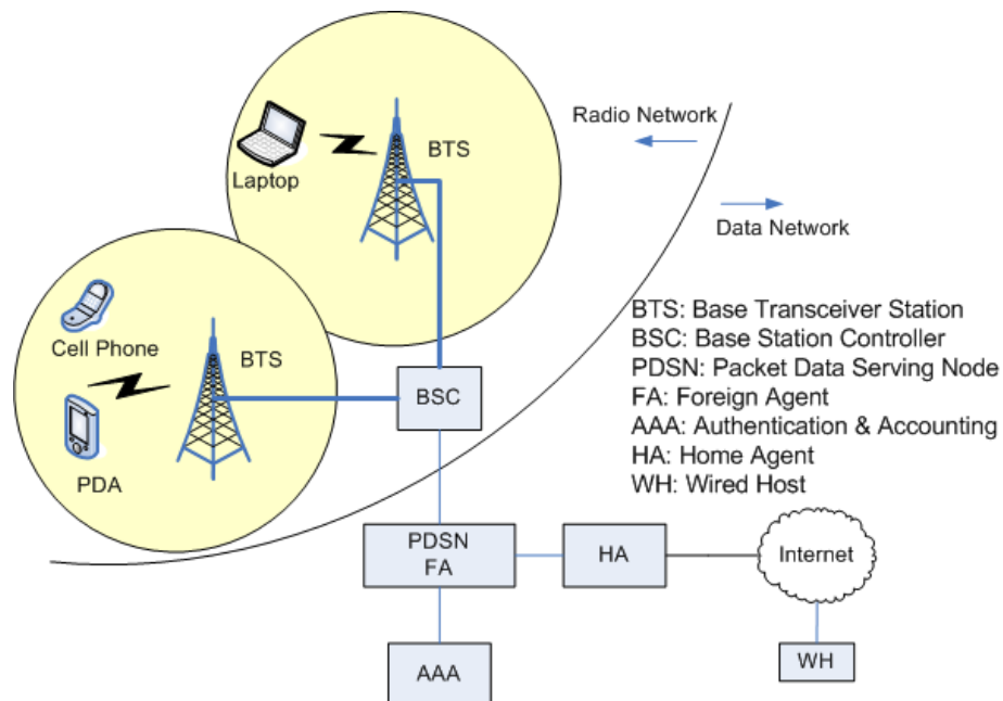
Figure 2.1: Network Architecture
