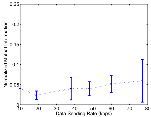
Figure 6.5: Impact of Channel Conditions on Wireless Scheduler
