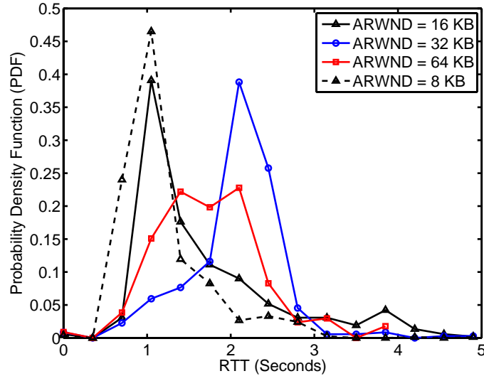
Figure 5-1: PDF of RTT for Different TCP ARWND
