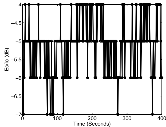
Figure 6-4: Sample E_c/I_o Signal
