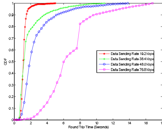
Figure 6-11: CDF of Round Trip Time for UDP CBR Experiments
