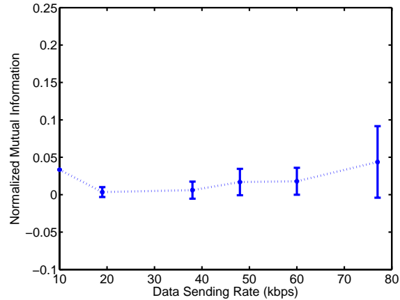
Figure 6-6: Impact of Sector Load on Wireless Scheduler
