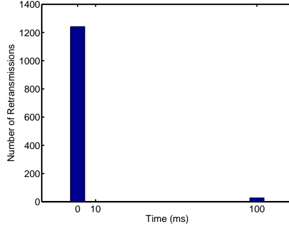
Figure 7-7: Histogram of Re-transmissions Versus Time Delay Since Last Ack Was Received
