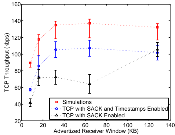
Figure 7-5: TCP Throughput as a Function of ARWND
