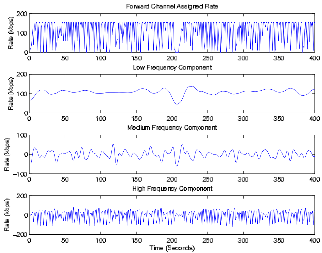
Figure 5.3: Wavelet Decomposition of a Sample Forward Channel Assigned Rate Signal
