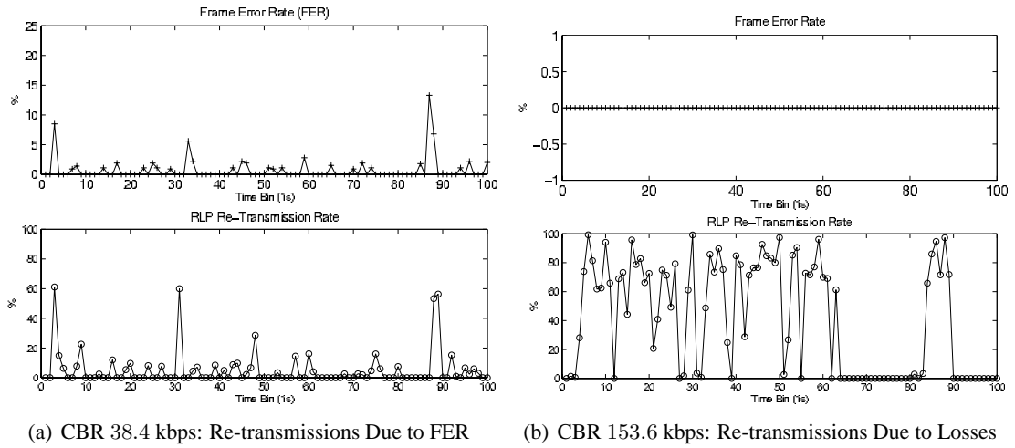
Figure 6-10: Sources of RLP Re-transmissions
