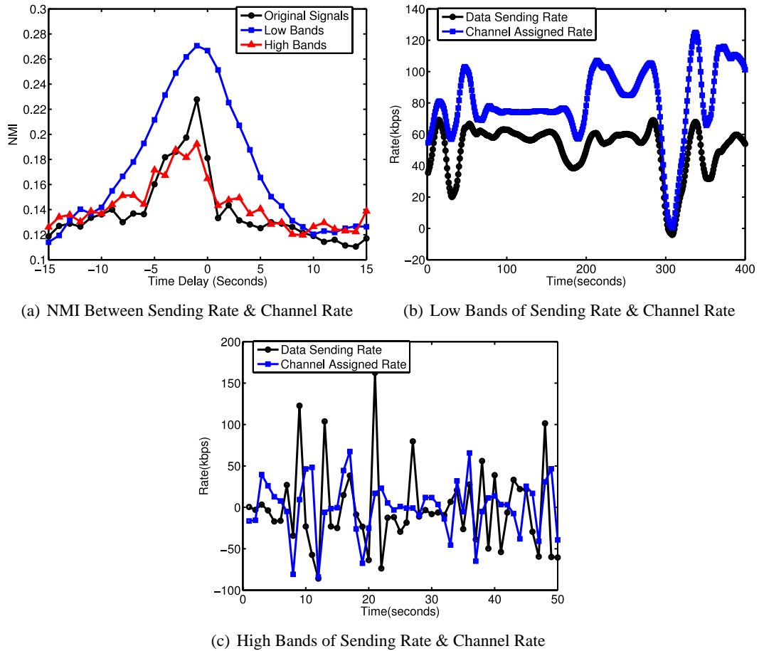
Figure 7-4: Coupling Between Sender and Wireless Scheduler
