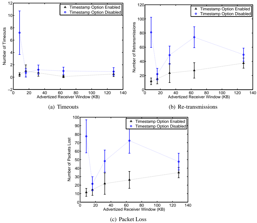
Figure 7-6: TCP timeouts, Re-transmissions and Packet Loss
