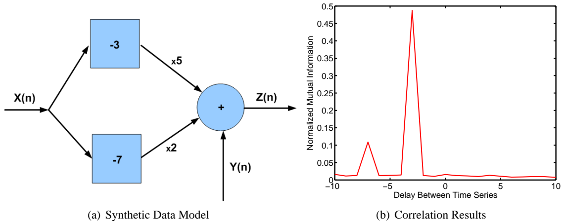
Figure 5-2: Correlation Results Using a Synthetic Data Model
