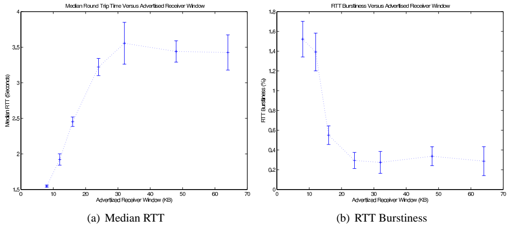
Figure 7-1: RTT Behavior as a Function of ARWND
