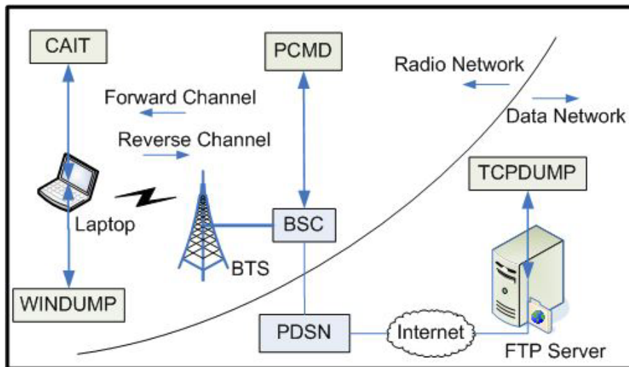
Figure 4-1: Experimental Setup
