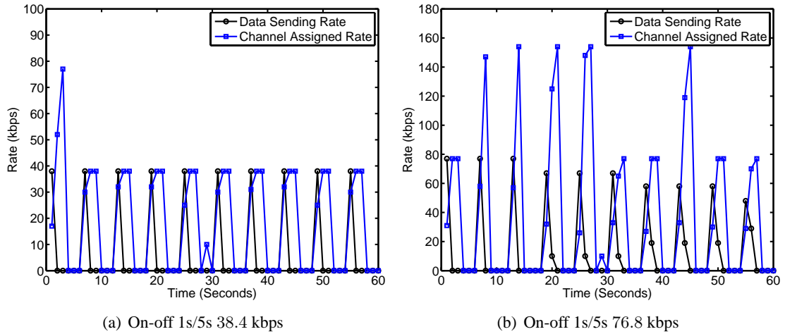
Figure 6-2: Wireless Scheduler Behavior at Short Time Scales
