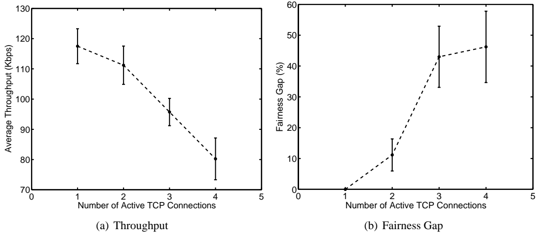
Figure 7-8: Impact of Sector Load on TCP
