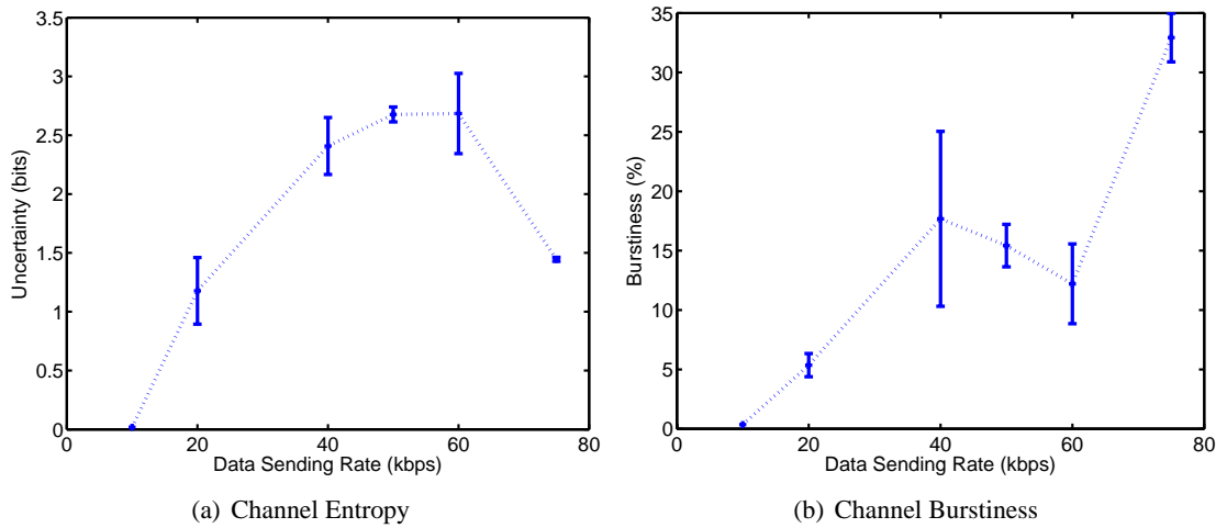
Figure 6.7: Properties of the Wireless Scheduler
