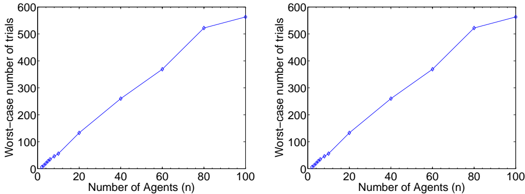
Fig. 12. Number of trials until convergence. Left – 5 time-slots, Right – 10 time-slots
