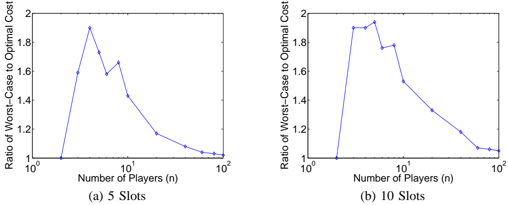
Fig. 4. Empirical Price-of-Anarchy based on synthetic worksets
