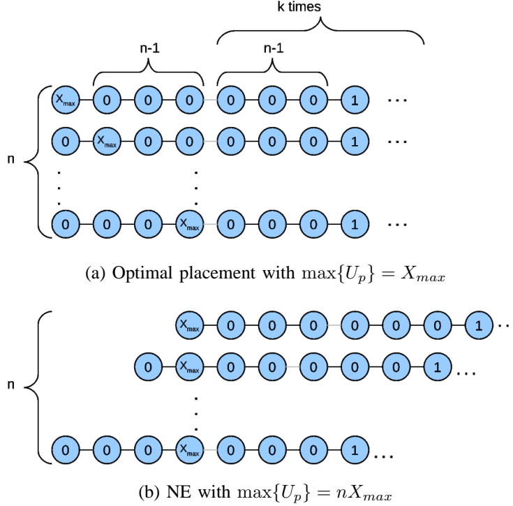
Fig. 3. Tight example for the PoA of the Bandwidth Trading Game
