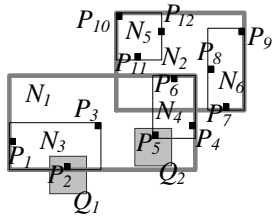
(a) Queries
