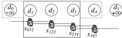
Figure 2.2 Example of signature chaining
