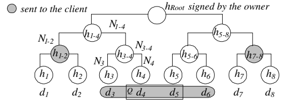
Figure 2.1 Example of Merkle Hash Tree
