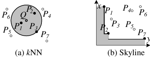
Figure 3.5 Alternative queries
