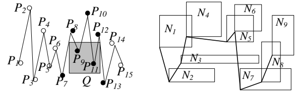
(a) Leaf Node (b) Internal Node Figure 2.3 Signature chains in the VR-tree
