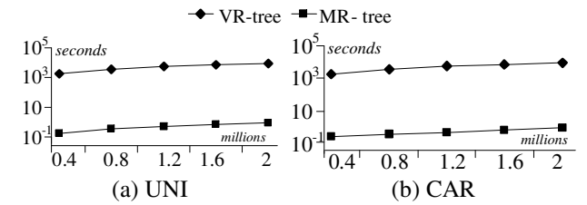
Figure 5.2 CPU time for authentication data vs. cardinality
