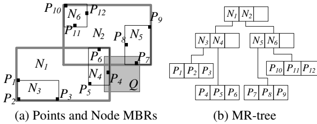
Figure 3.3 Example range query
