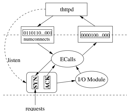
Figure 8: Modified thttpd web server using ECalls and the I/O module: ECalls monitors both the number of open connections ( numconnects ) and the buffer fill level of the listen queue with completed requests (ACK-queue) to determine the size of the listen queue with incomplete requests (SYN-queue).
