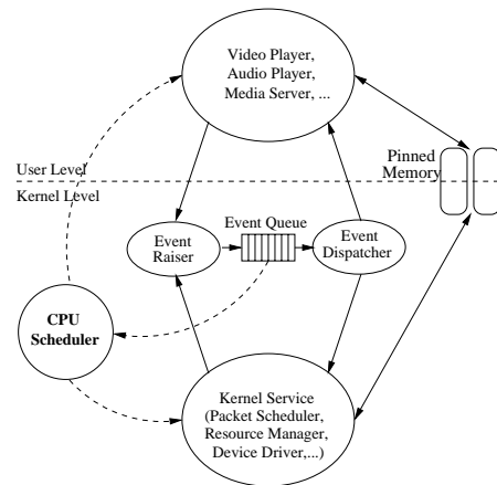
Figure 1: Architecture of ECalls.
