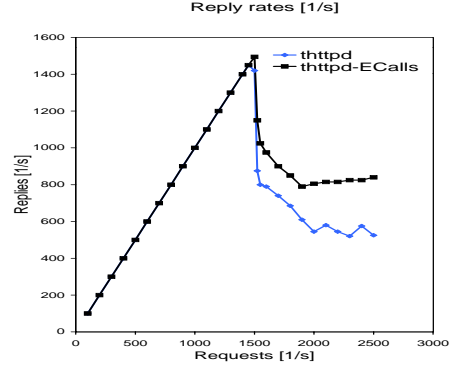
Figure 6: Reply rates for both the tthttpd web server and the modified tthttpd web server using ECalls and the I/O event delivery module.
