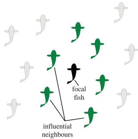
Figure 5. In the topological distance model, a set of animals nearest the focal animal (black) is considered to comprise influential neighbours (green). Animals outside this inner grouping (grey) are not considered by the focal animal.
