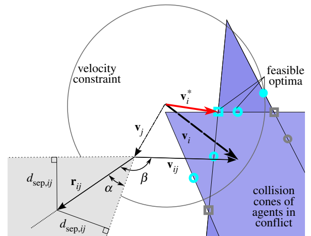
Figure 6. The grey cone with dashed borders depicts the anatomy of a collision cone for an agent that is not in a conflict: \alpha < \beta indicates that v_{ij} falls outside the collision cone. The blue cones with solid borders depict collision cones for agents in conflict; potential optima are shown that are within the maximum velocity constraint (cyan) and as well as those that are infeasible (grey) at locations 1 and 2 on a single collision cone (open and closed circles, respectively) and location 3 on the intersection of collision cones (square).
