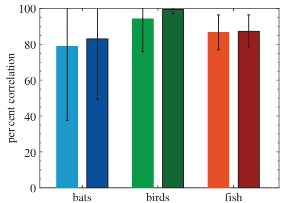
Figure 9. The per cent correlation for each species with (darker bar with border on the right) and without (lighter bar on the left) acceleration limits applied to the DRCA optimal velocity. The error bars indicate one standard deviation above and below the mean per cent correlation (error values above 100% are not shown).
