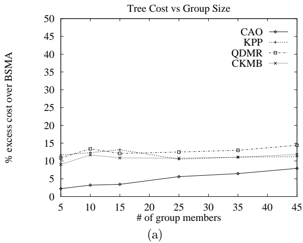
Figure 5. Tree cost and execution time versus group size: network size=50, delay bound=30 ms.
