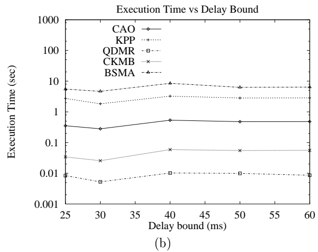
Figure 6. Tree cost and execution time versus delay bound: network size=50, group size=15.
