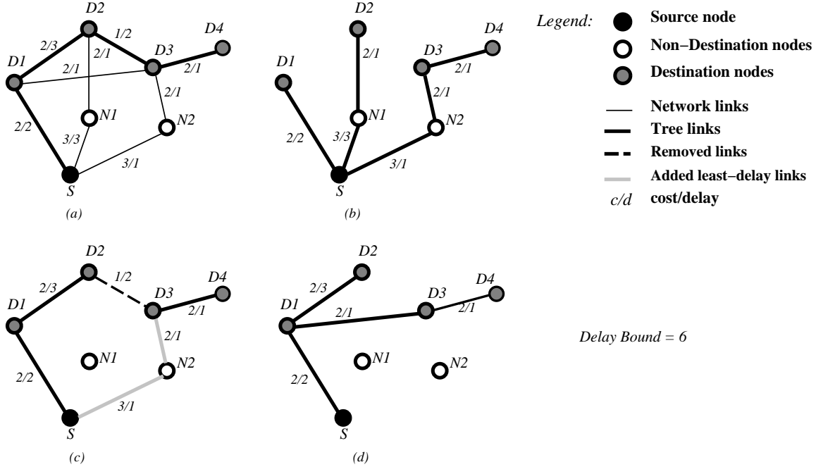
Figure 1. Example to show difference between DDMC and QDMR: (a) Example network and DDMC tree; (b) Least-delay tree (LDT); (c) DDMC+LDP tree; (d) QDMR tree.
