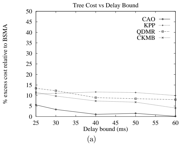
Figure 6. Tree cost and execution time versus delay bound: network size=50, group size=15.
