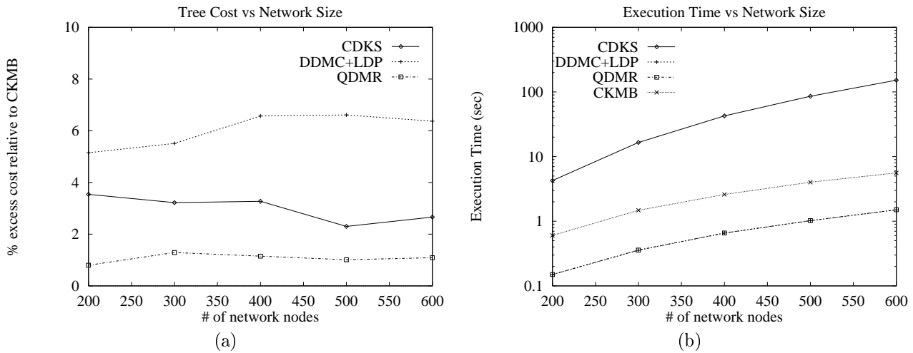
Figure 7. Tree cost and execution time vs network size: group size=10% of network size, delay bound=30 ms.
