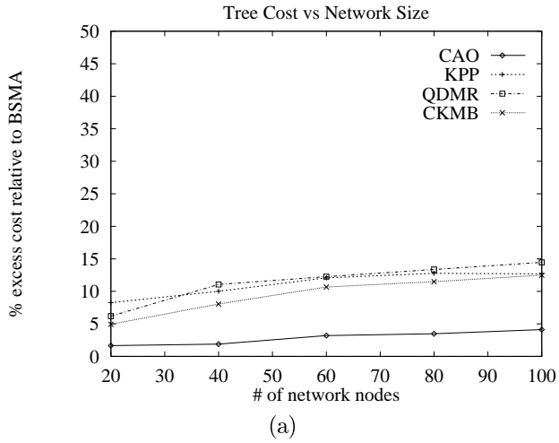
Figure 4. Tree cost and execution time versus network size: group size=10, delay bound=30 ms.
