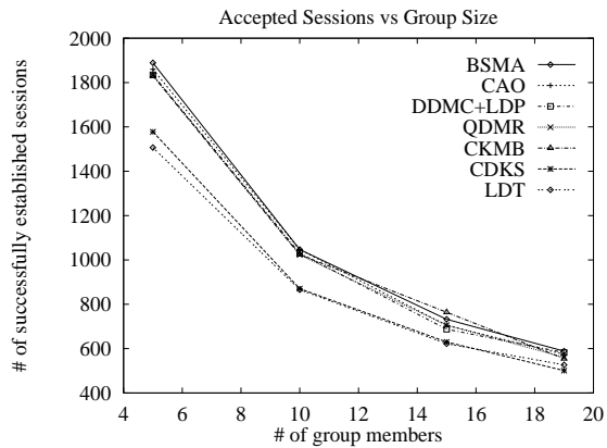
Figure 8. Number of admitted sessions versus group size: network size=20, delay bound=30 ms.
