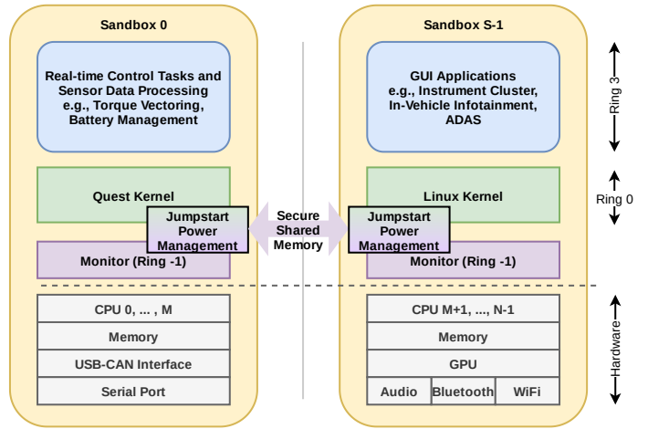
Figure 1. Structure of the Jumpstart vehicle management system
