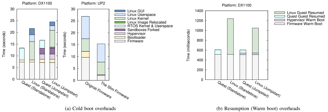
Figure 6. Summary of startup delays in all scenarios
