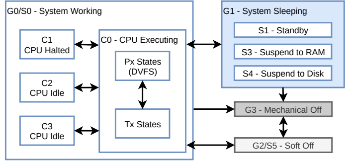
Figure 3. ACPI power states
