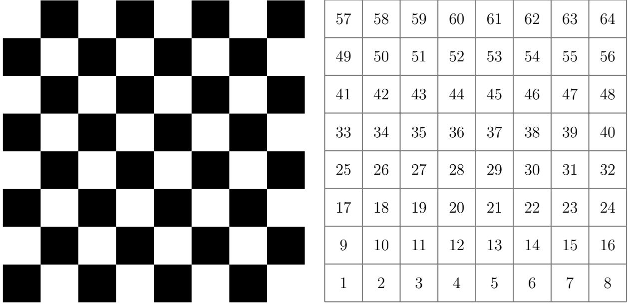
Figure 1: A chess board (on the left) and the numbering of its squares (on the right). Initially, all White pieces are placed in squares 1, 2, ..., 16 and all Black pieces are placed in squares 49, 50, ..., 64.
