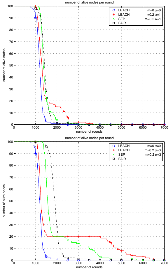
Fig. 7. Comparison between LEACH and SEP in the presence of heterogeneity: (top) m = 0.2 and \alpha = 1 , and (bottom) m = 0.2 and \alpha = 3 .
