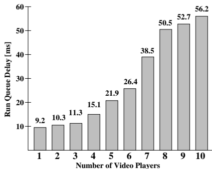
Figure 2: Average run queue delays for a number of video players that have to compete with each other and with another real-time process (running in an endless loop) for the CPU.
